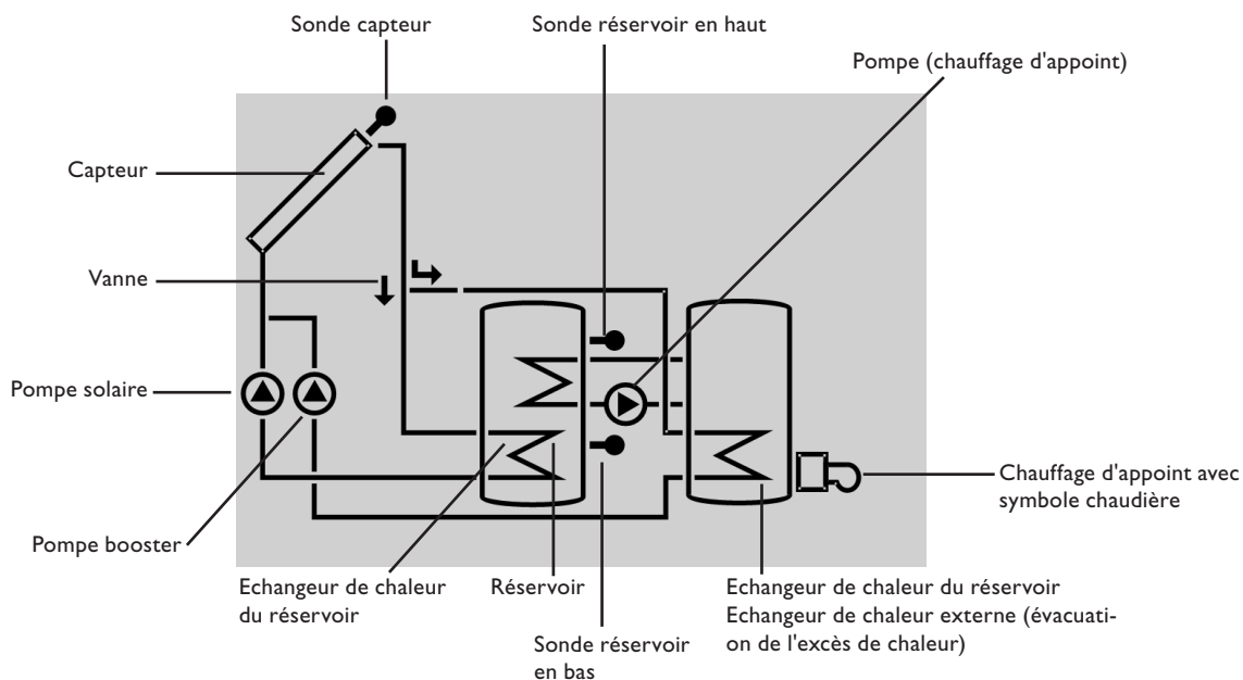
Le System-Screen
